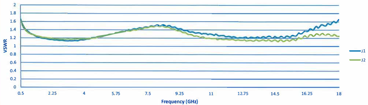
VSWR @ -20 dB
