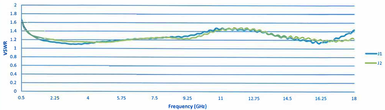
VSWR @ -20 dB
