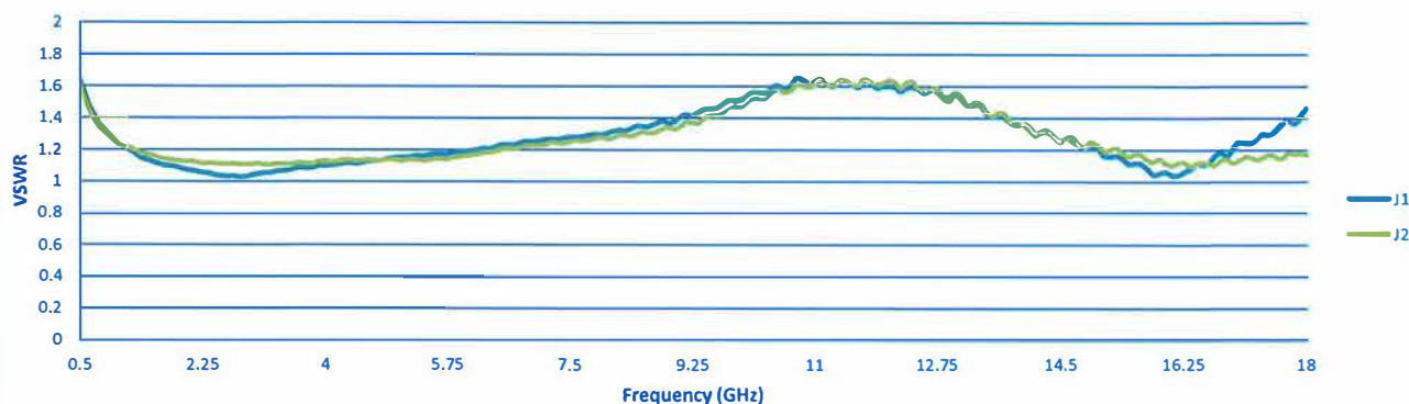
VSWR @ -20 dB
