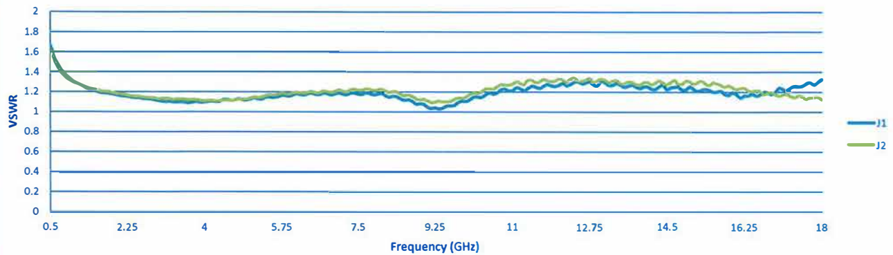
VSWR @ -20 dB
