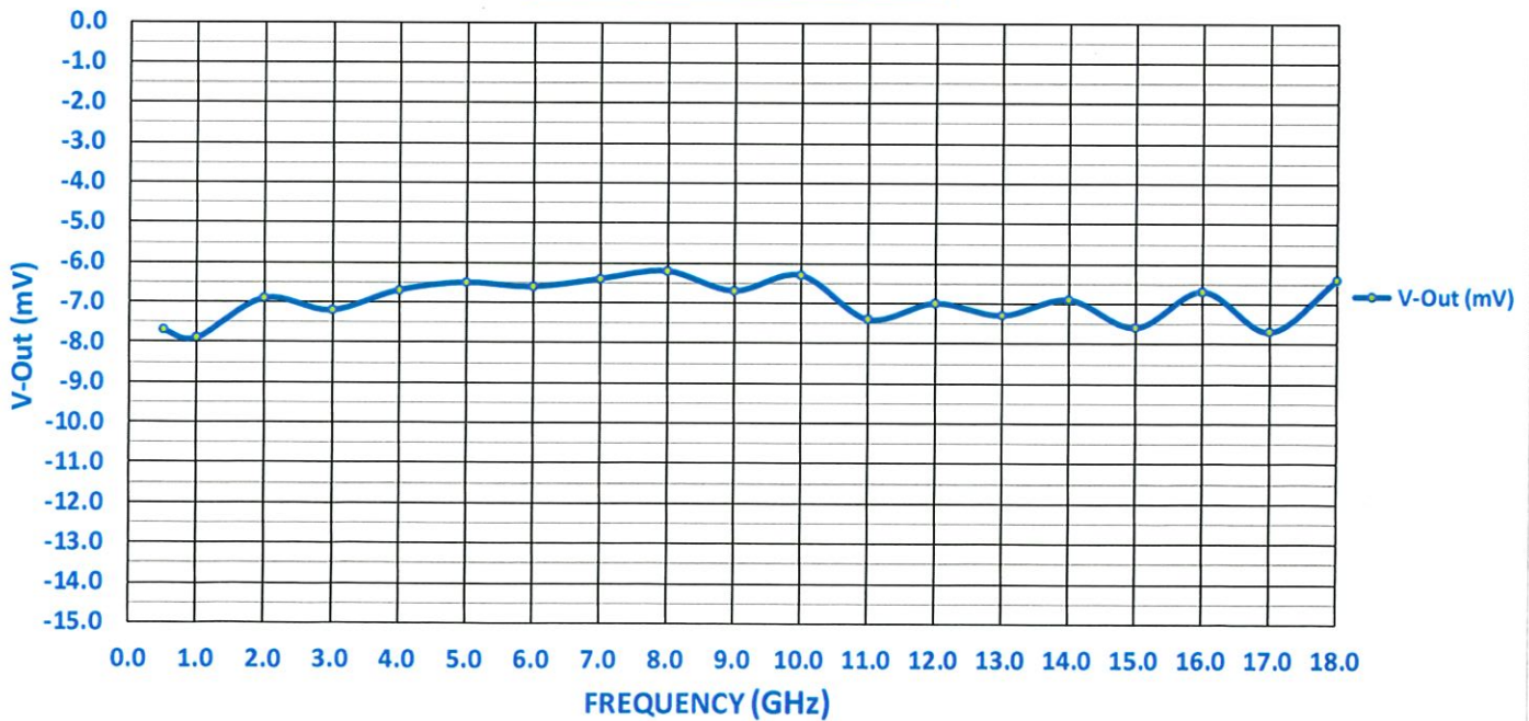
Detector V-Out VS frequency
