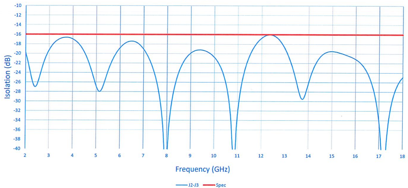
Isolation
