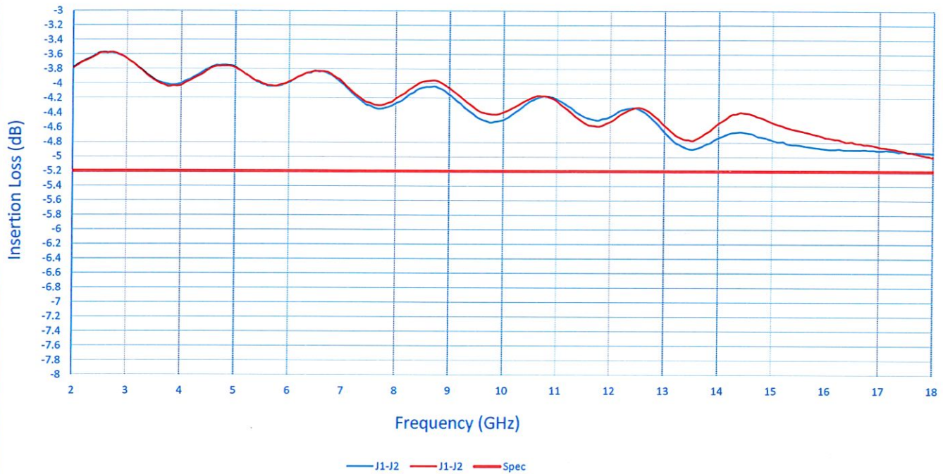
Insertion Loss
