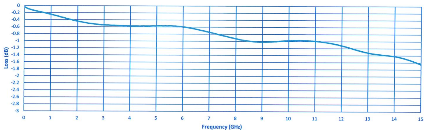
Insertion Loss
