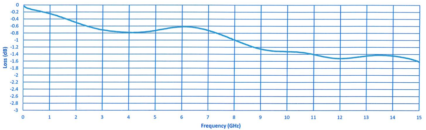
Insertion Loss
