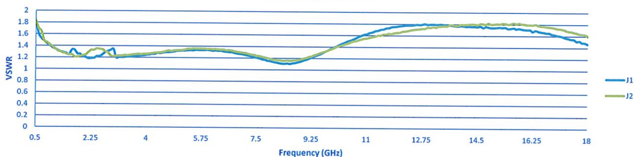
VSWR @ -20 dB
