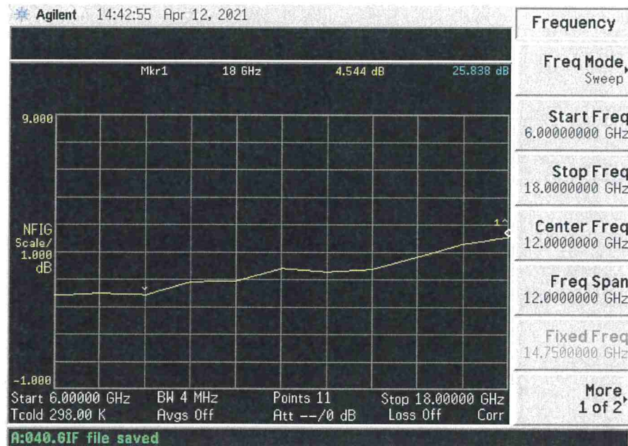
OP1dB Plot
