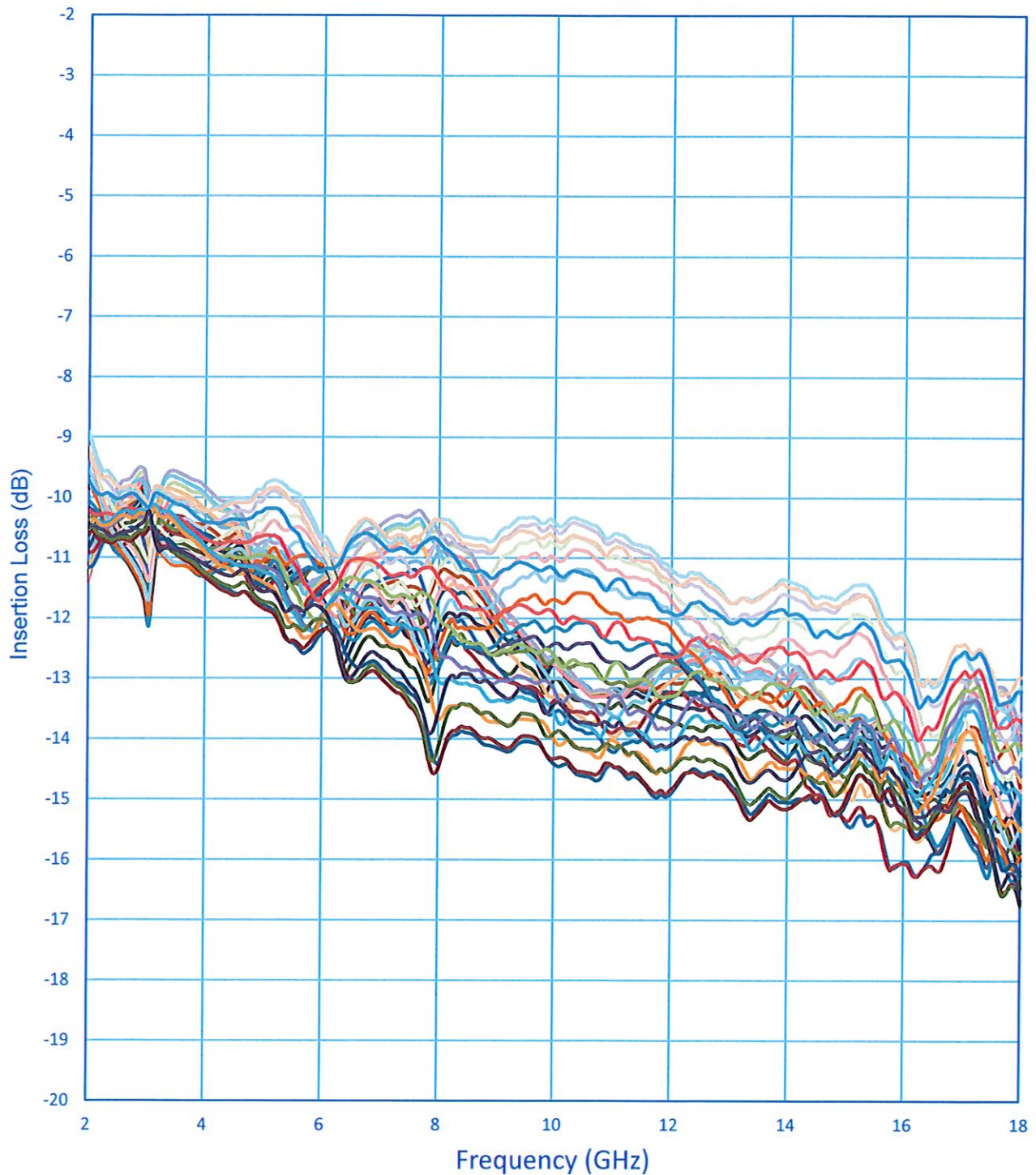
Insertion Loss Vs. Frequency
