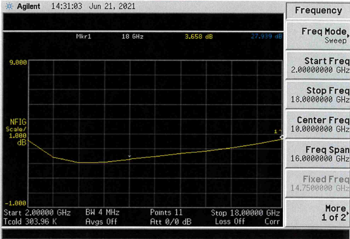
Noise Figure Plot
