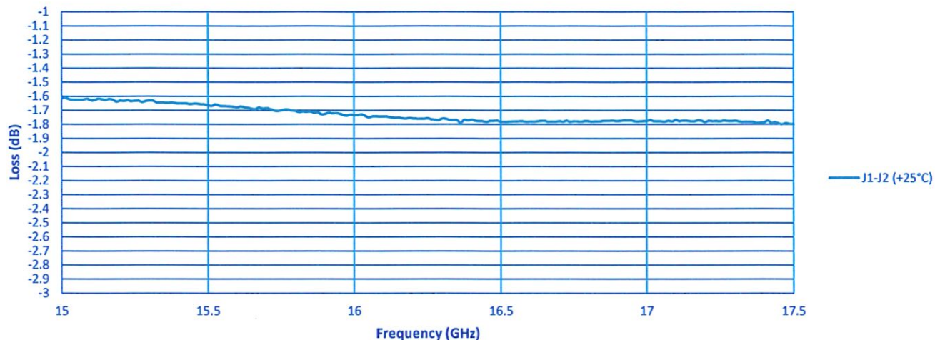
Insertion Loss
