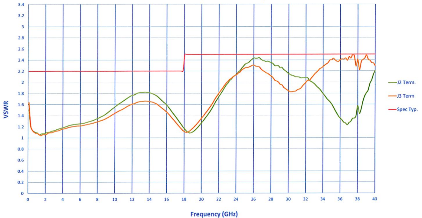
VSWR (Termination)
