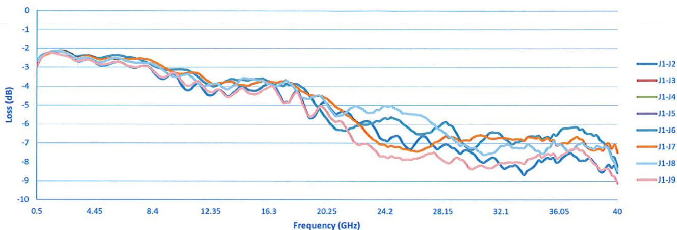
Insertion Loss
