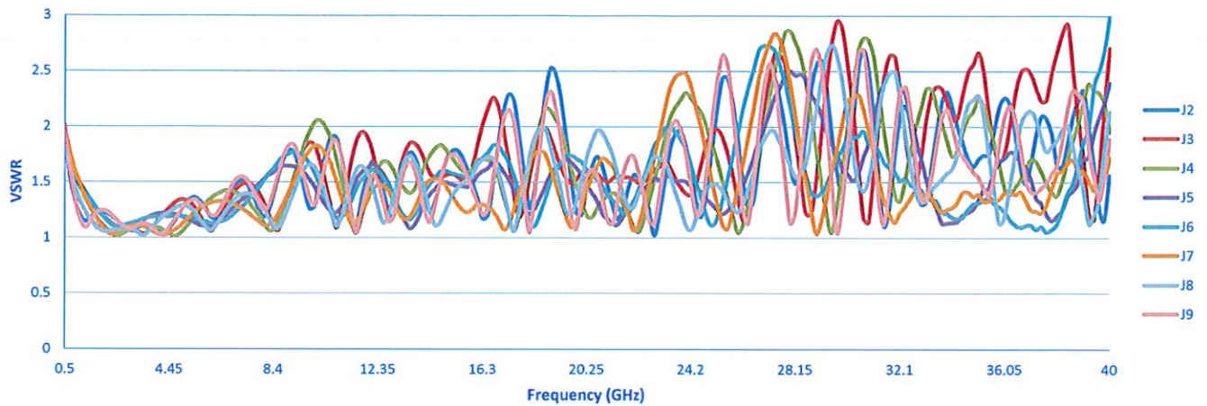
Output VSWR (On)
