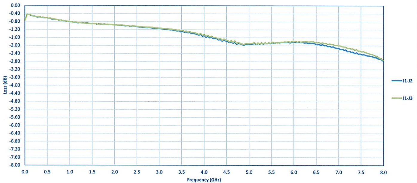
Insertion Loss
