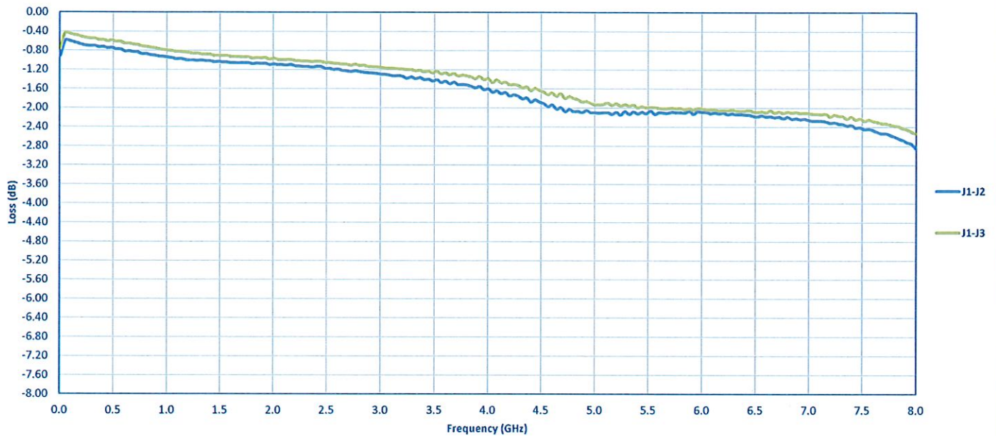
Insertion Loss
