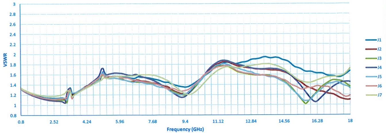
VSWR In
