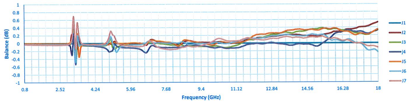
Amplitude Balance
