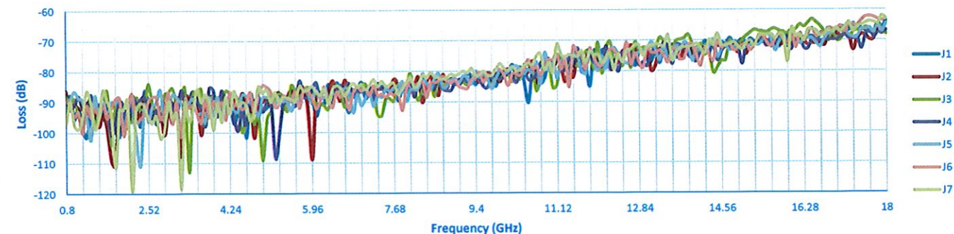
Isolation
