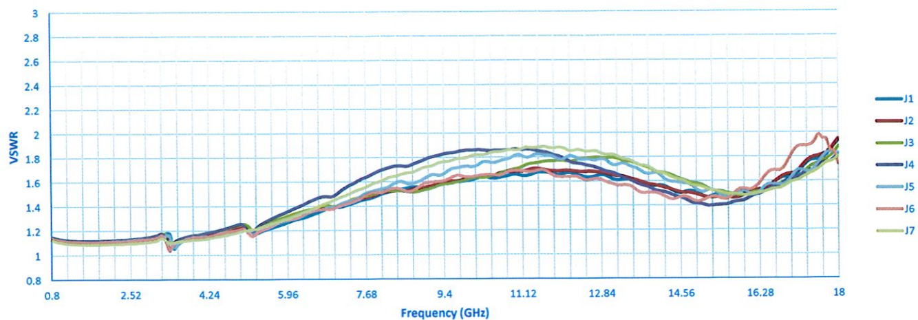
VSWR Off
