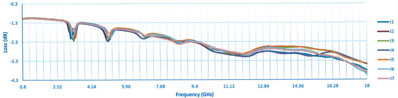
Insertion Loss
