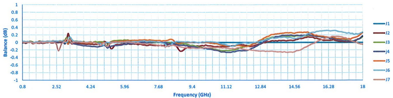
Amplitude Balance
