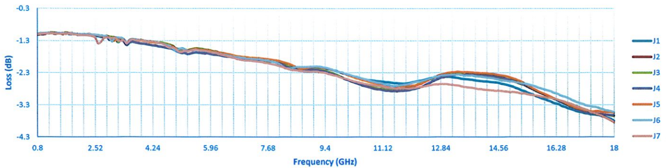
Insertion Loss
