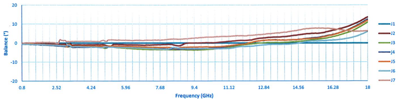
Phase Balance
