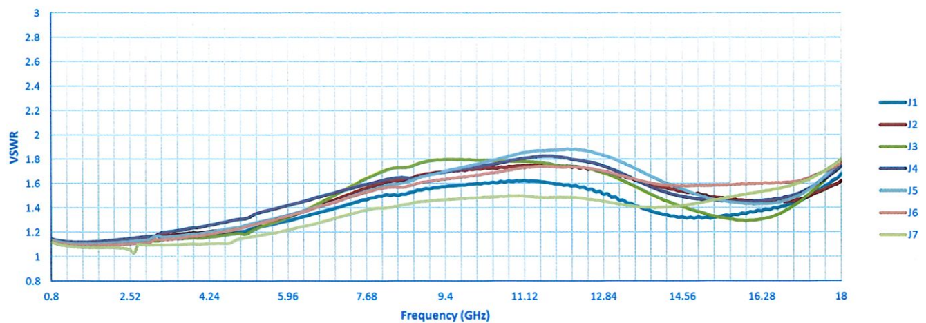
VSWR Off
