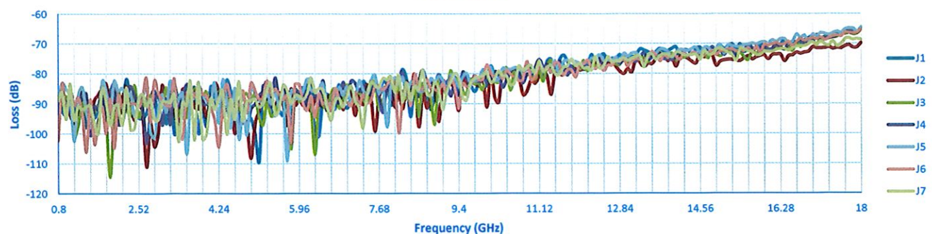
Isolation
