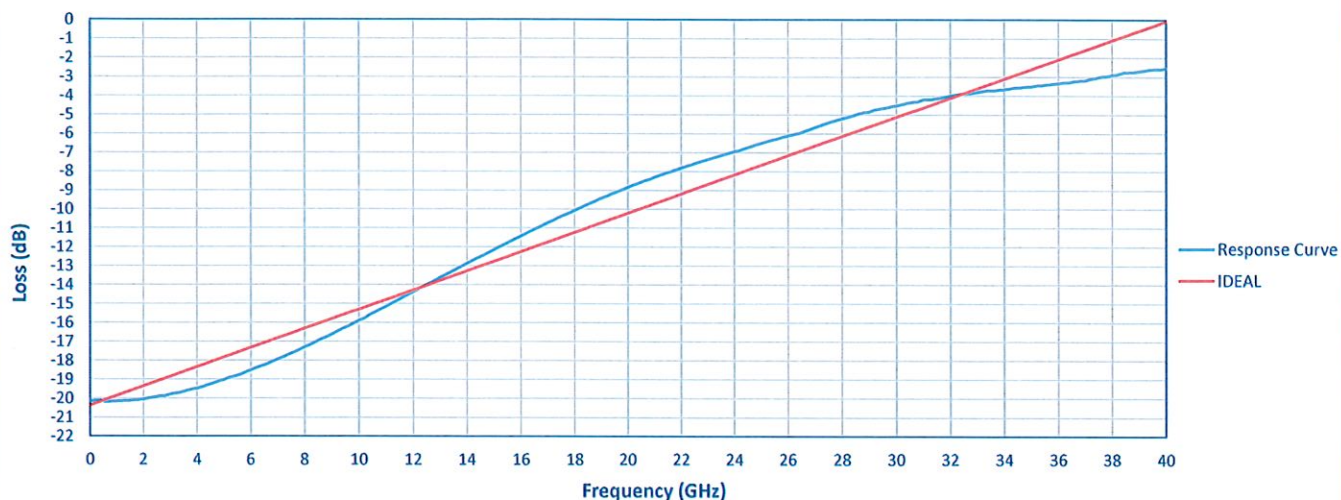
Insertion Loss
