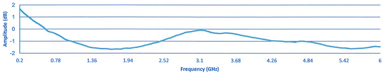
Gain Flatness
