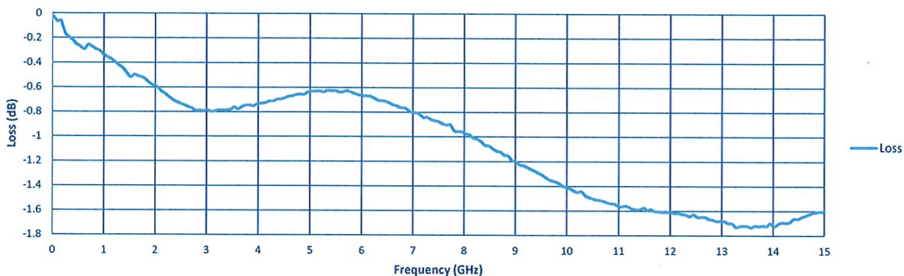
Insertion Loss
