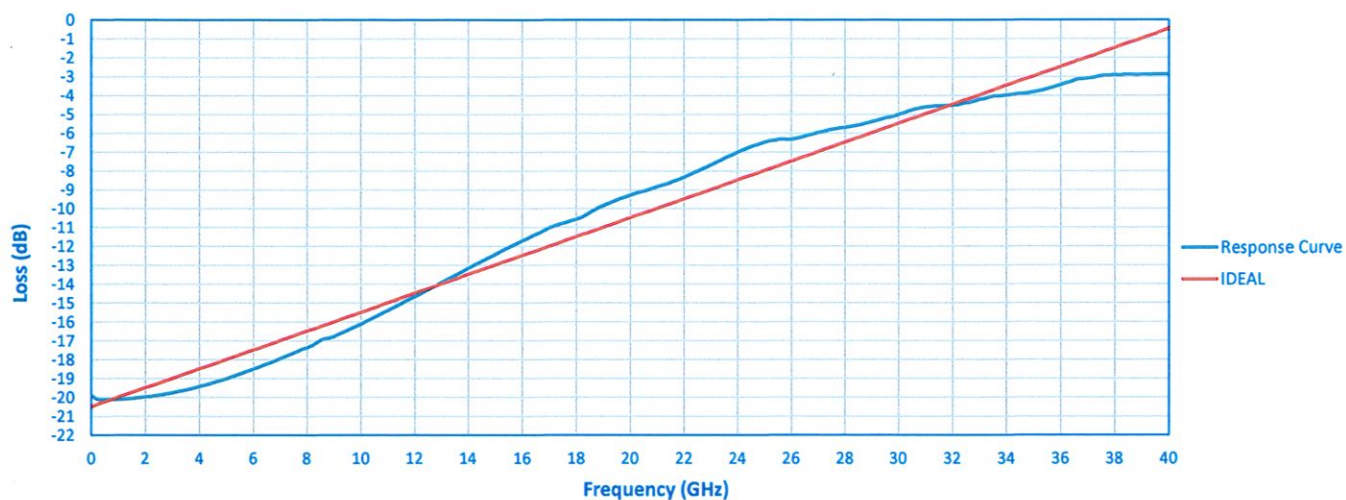
Insertion Loss
