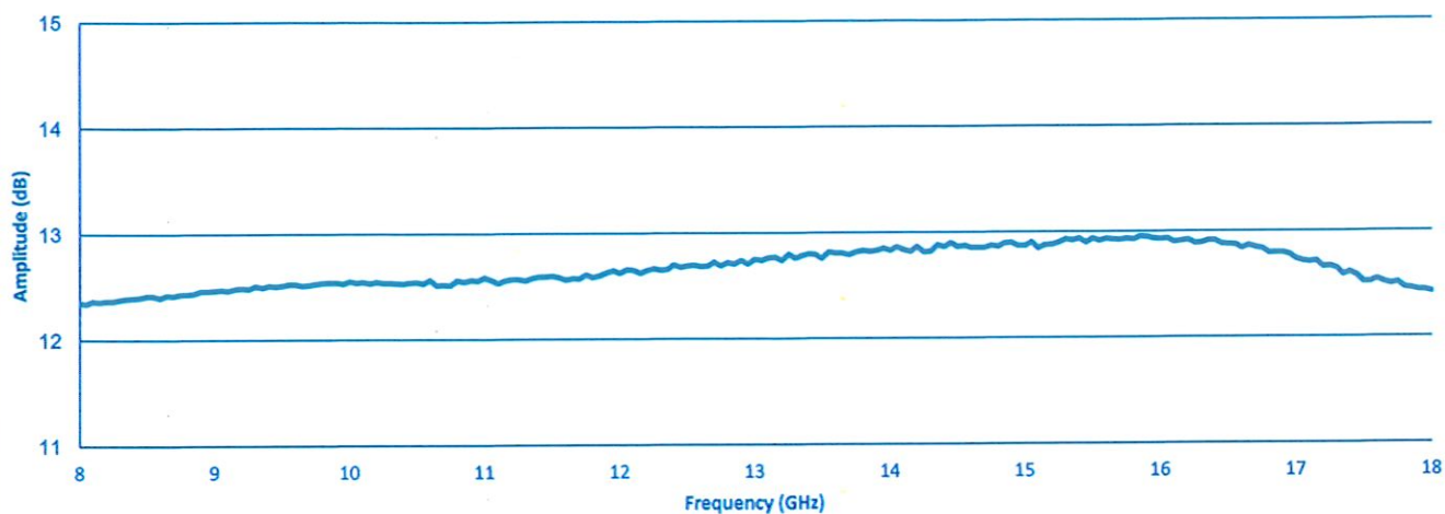
Gain
