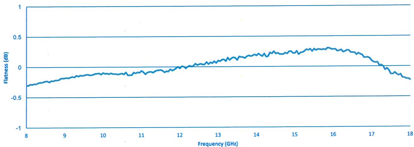
Gain Flatness
