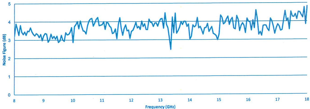
Noise Figure
