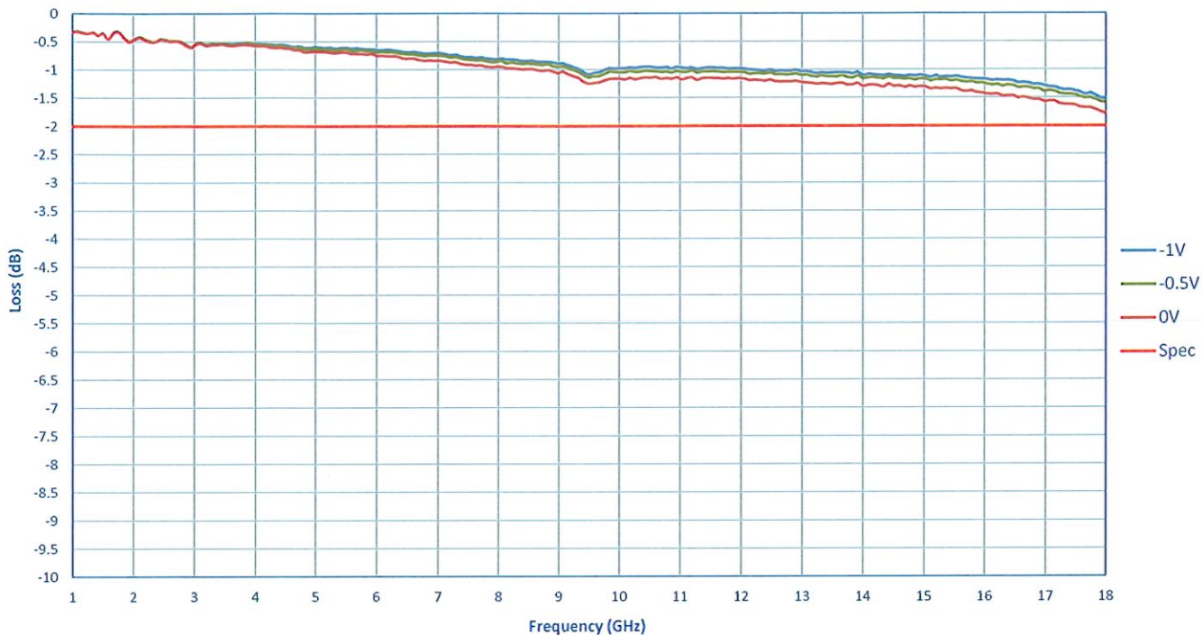
Insertion Loss
