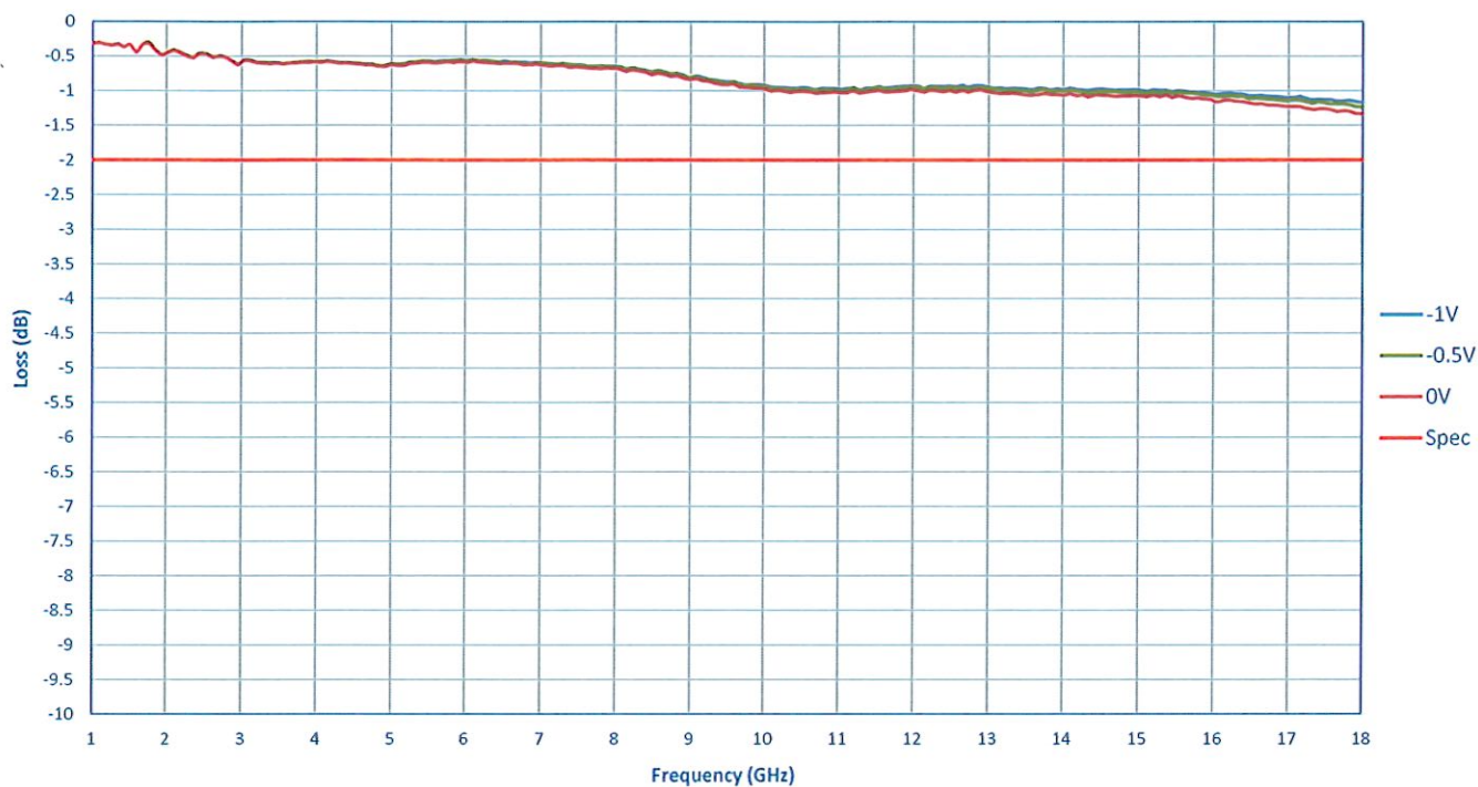
Insertion Loss
