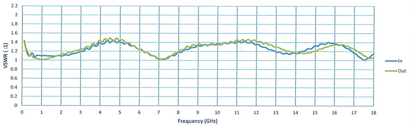
VSWR @ -20 dB
