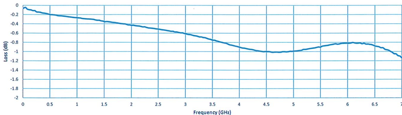
Insertion Loss
