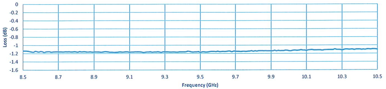
Insertion Loss
