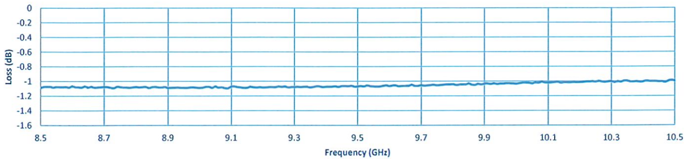
Insertion Loss
