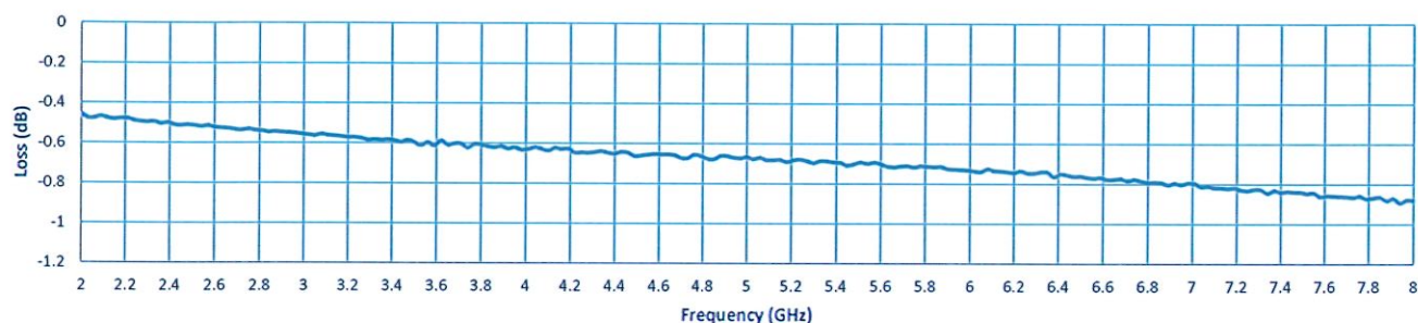
Insertion Loss
