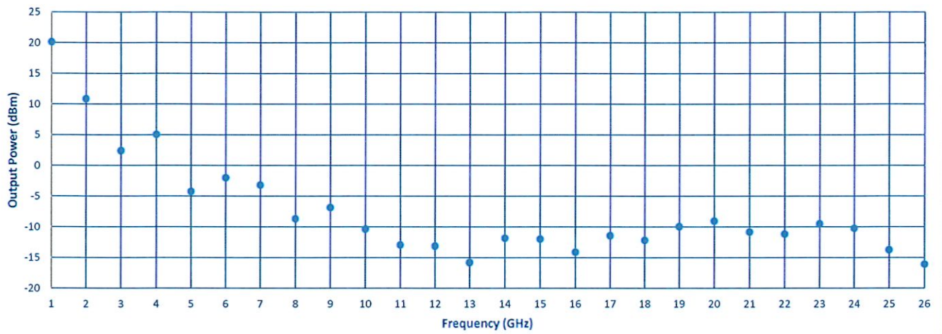
1 GHz Comb Generator Output
