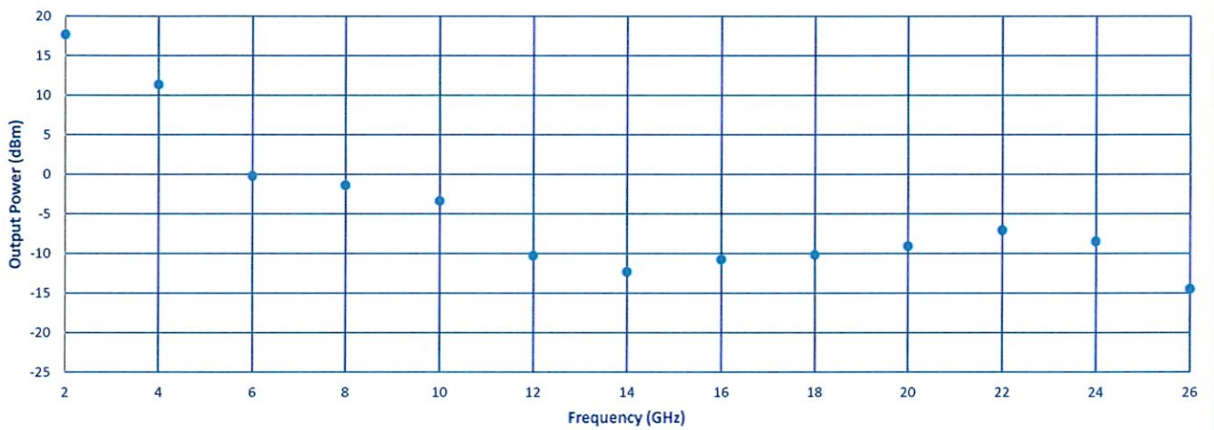
2 GHz Comb Generator Output
