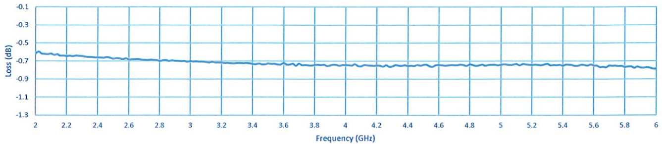
Insertion Loss
