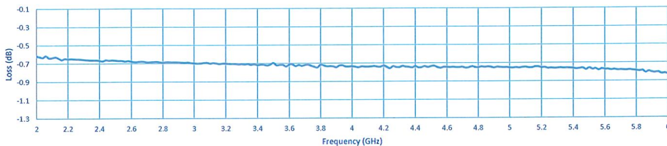
Insertion Loss
