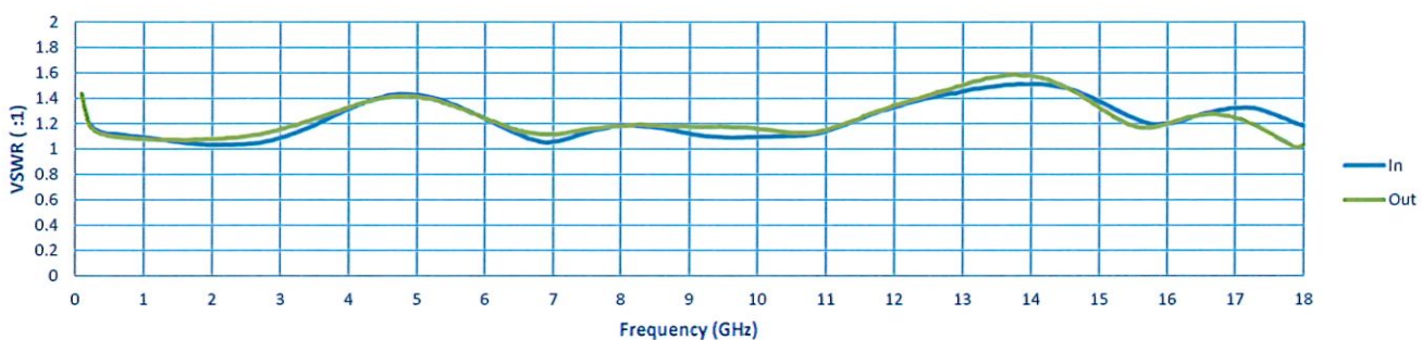
VSWR @ -20 dB
