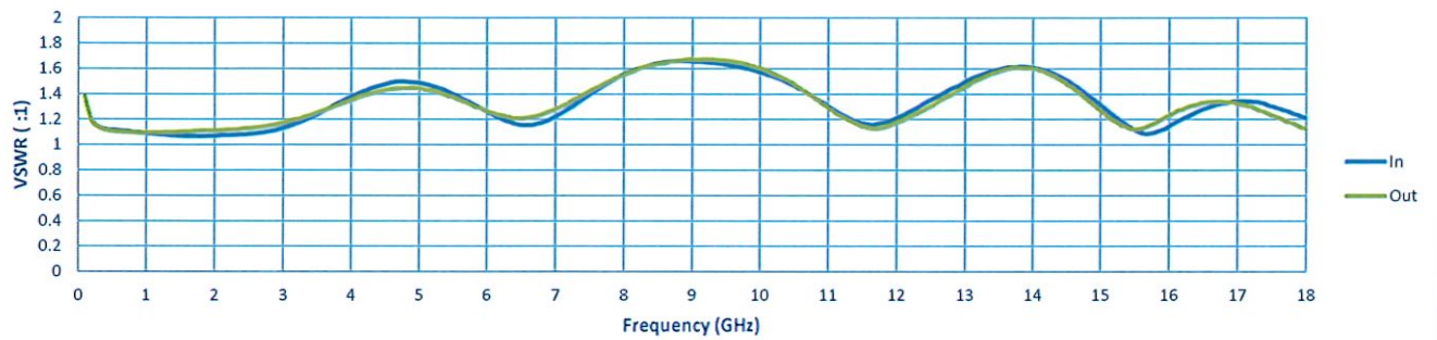
VSWR @ -20 dB
