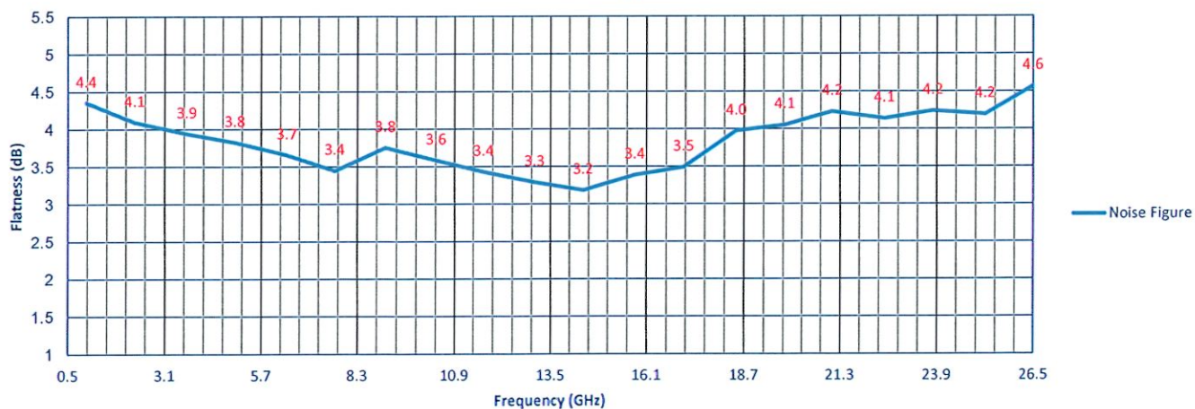
Noise Figure
