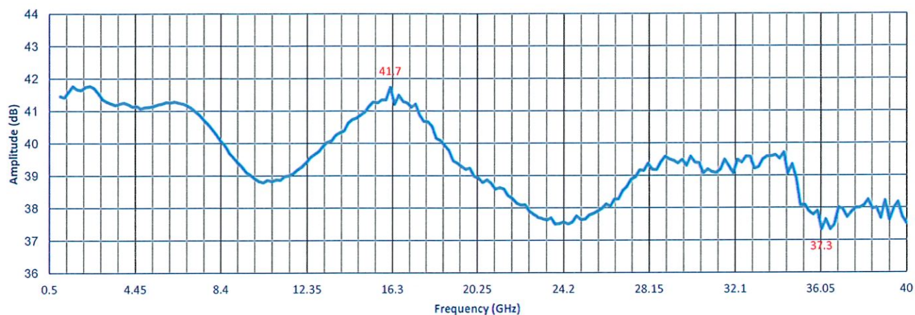
Gain
