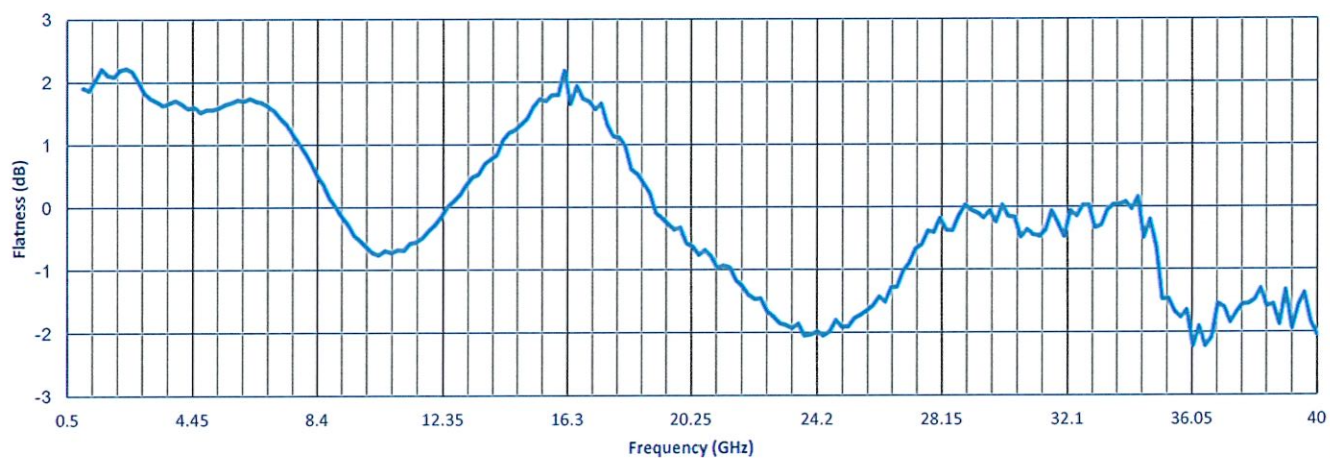
Gain Flatness
