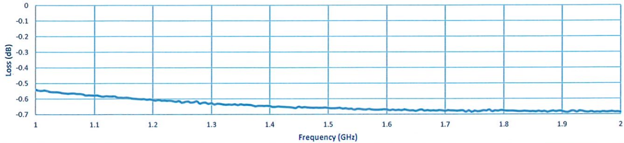
Insertion Loss @ -10dBm
