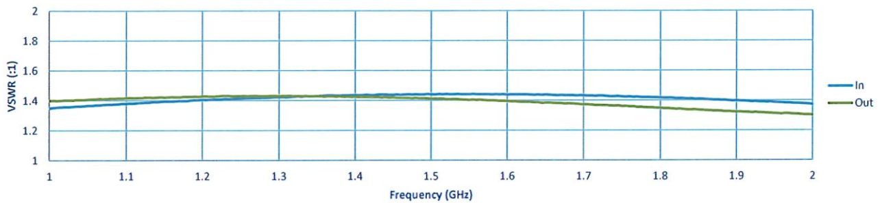
VSWR @ -10 dBm
