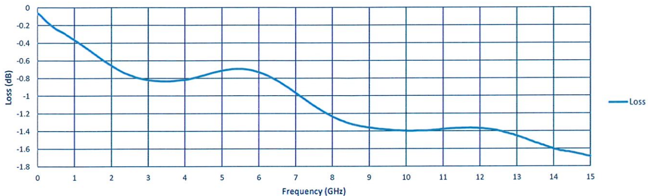
Insertion Loss
