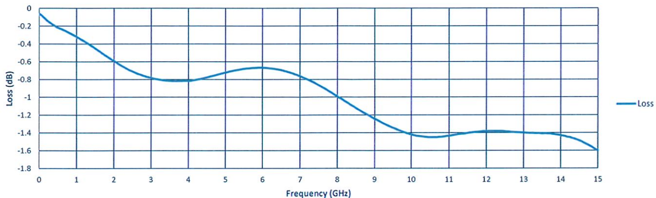
Insertion Loss
