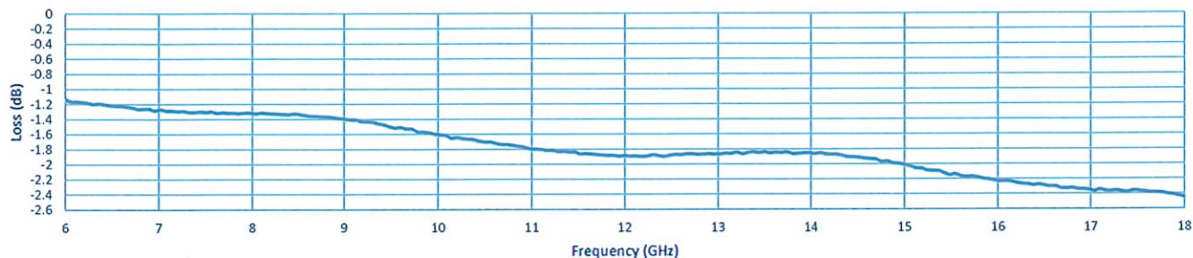
Insertion Loss
