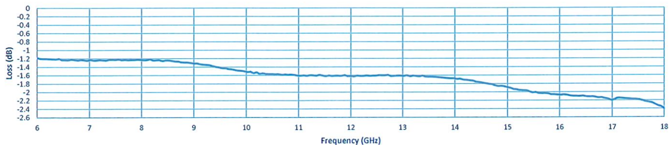
Insertion Loss
