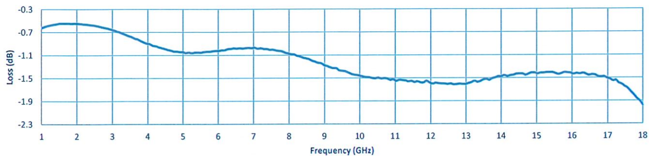
Insertion Loss
