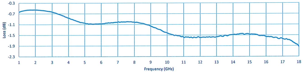
Insertion Loss
