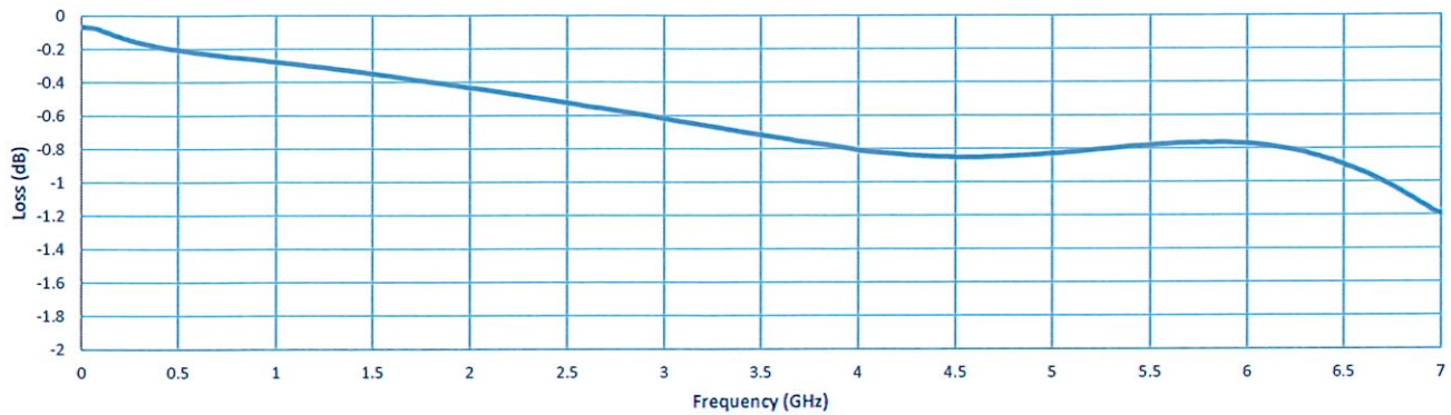
Insertion Loss
