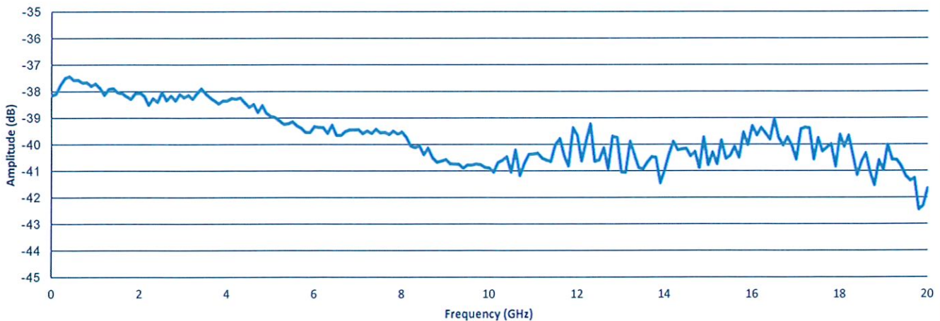
Reverse Isolation
