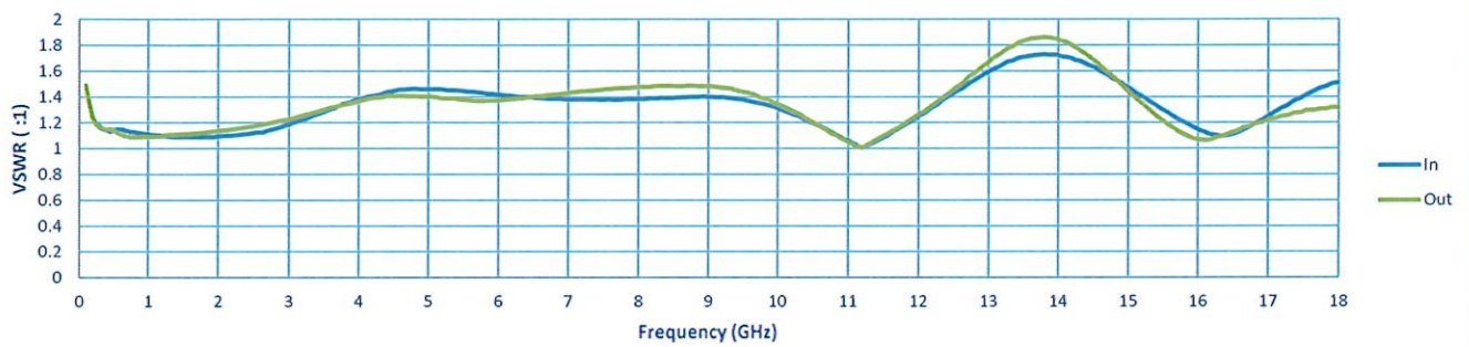
VSWR @ -20 dB
