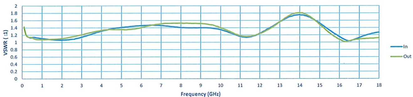
VSWR @ -20 dB
