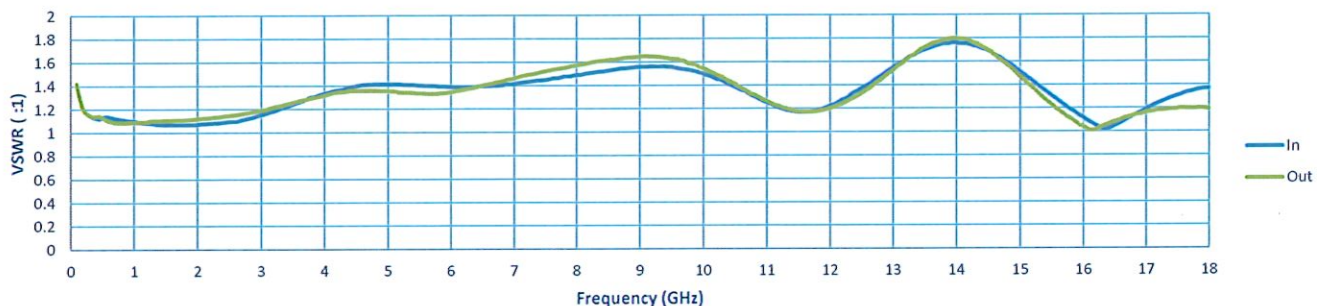
VSWR @ -20 dB
