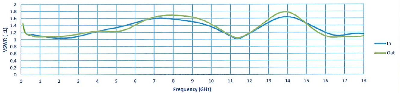
VSWR @ -20 dB
